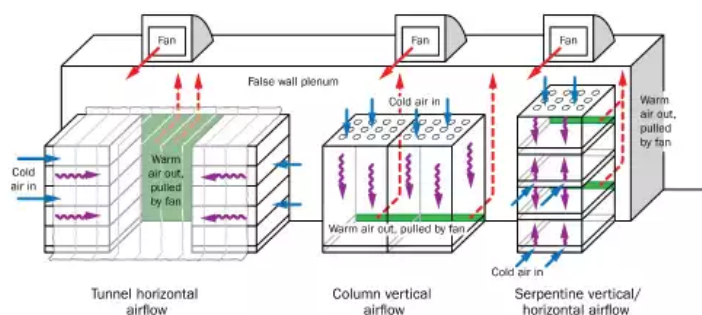
Figure 1. Cold, refrigerated air (blue arrows) is pulled through containers by high-capacity fans in a false wall plenum within a cold storage. These fans create a partial vacuum and pull air through strategically located openings (green shading) in the plenum. Produce cools primarily by the convective action of high-speed cold air, when it picks up field heat from warm produce (purple arrows) as it passes around the produce. The warmed air (red arrows) is then blown back into the cold storage to the evaporator coils of the refrigeration system to be re-cooled.
