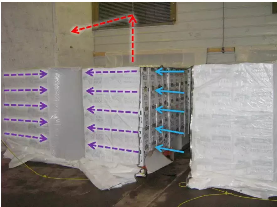
Figure 2. This tunnel horizontal airflow system has high-capacity fans inside a plenum (located behind the pallets) that pull refrigerated air (blue arrows) from the room horizontally through produce boxes. Warmed air (purple then red arrows) then travels through a "tunnel" created between the pallets and into the plenum, where it is directed back into the storage room (red arrows) towards the evaporator coils to be re-cooled. Pallets are cooled in pairs. Plastic sheeting sucks tightly against the boxes and tunnel. Sheetting is swung into place with cords attached to the ceiling.
