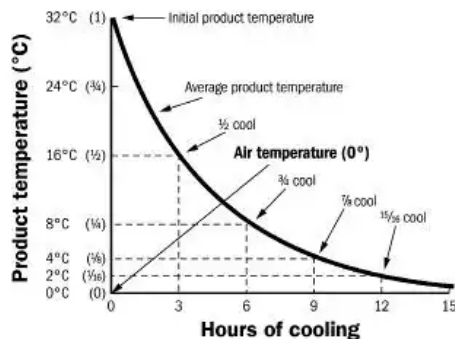
Figure 5. Time-temperature relationship for cooling produce.
